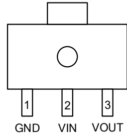
ET533XXC(SOT89-3)
