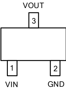
ET533XXE(SOT23-3)
