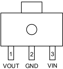
ET533XXD(SOT89-3)
