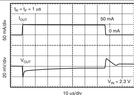
Figure 22. TLV70018 Load Transient Response
