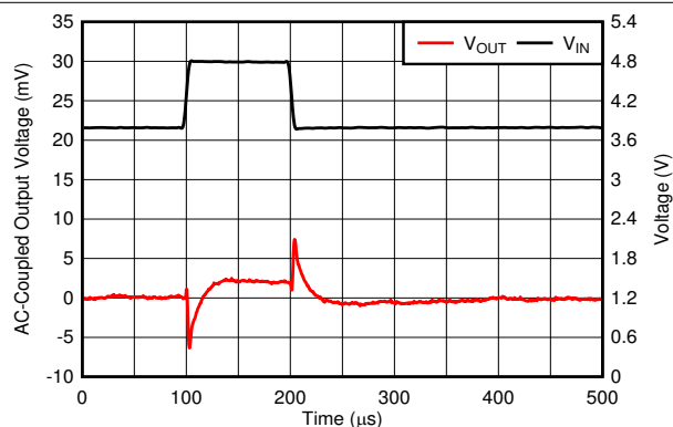
Figure 6-38. Line Transient
