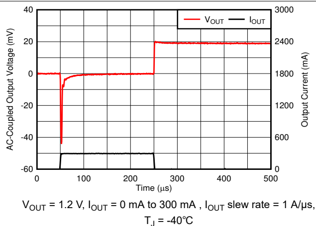
Figure 6-51. Load Transient
