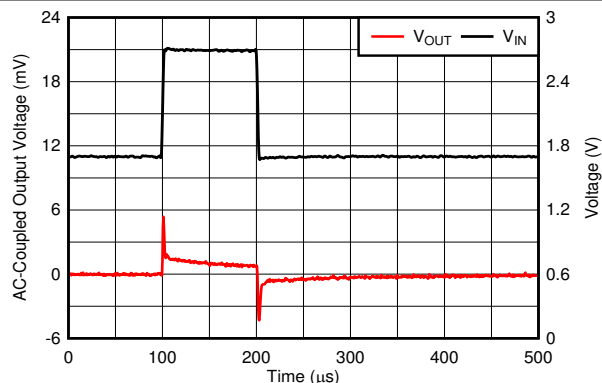
Figure 6-28. Line Transient
