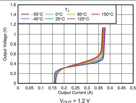
Figure 6-22. Foldback Current Limit vs I_{\text{OUT}} and Temperature
