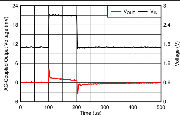
Figure 6-26. Line Transient
