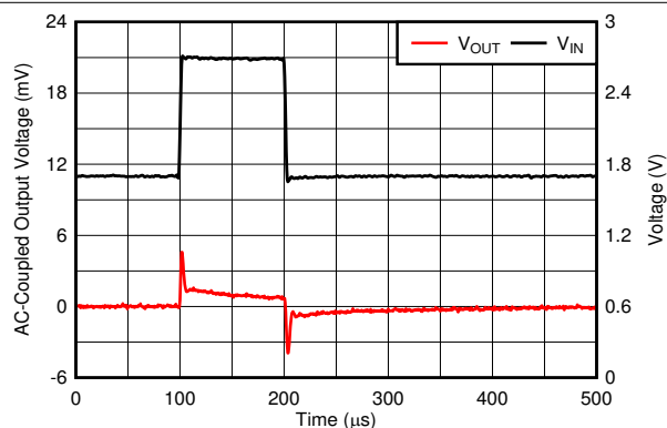
Figure 6-26. Line Transient
