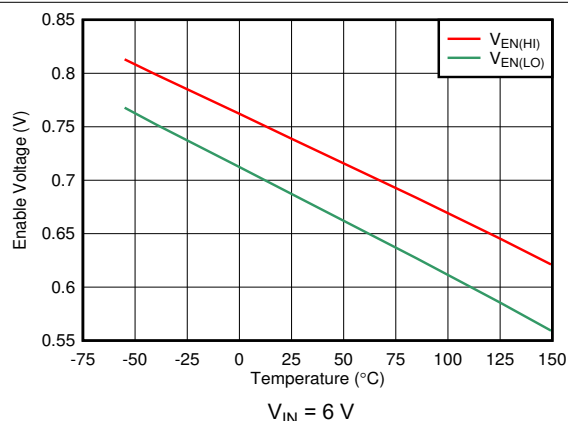
Figure 6-21. V_{\text{EN(HI)}} and V_{\text{EN(LO)}} Thresholds vs Temperature
