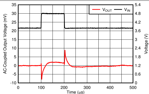
Figure 6-37. Line Transient
