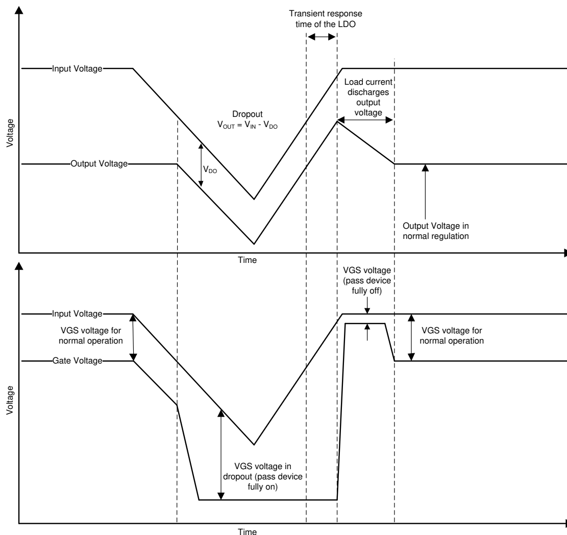
Figure 8-4. Line Transients From Dropout
