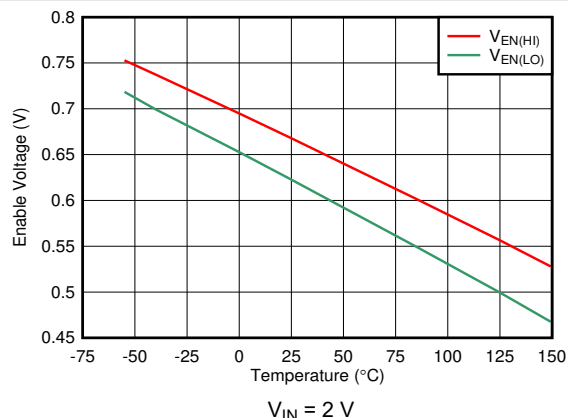
Figure 6-20. V_{\text{EN(HI)}} and V_{\text{EN(LO)}} Thresholds vs Temperature
