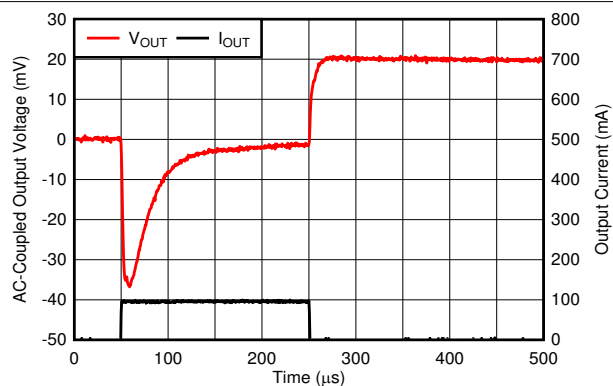
Figure 6-56. Load Transient
