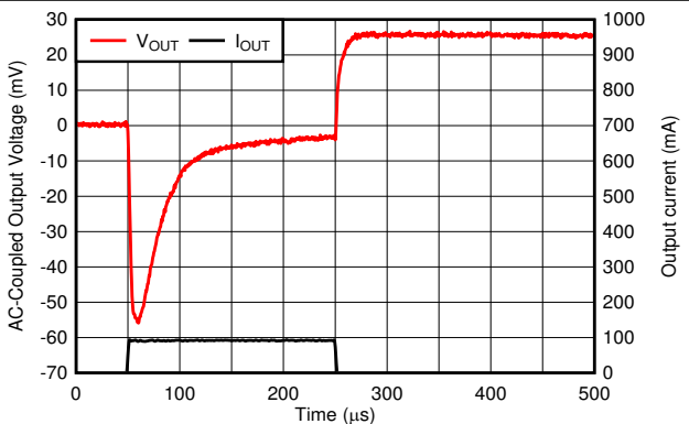
Figure 6-56. Load Transient
