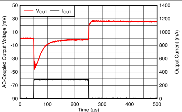
Figure 6-58. Load Transient
