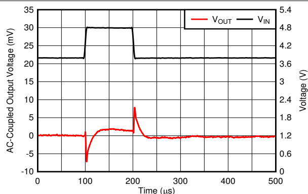
Figure 6-38. Line Transient
