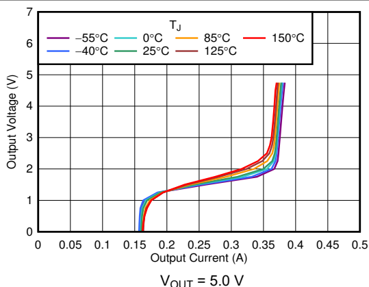
Figure 6-23. Foldback Current Limit vs I_{\text{OUT}} and Temperature
