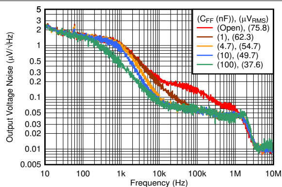
Figure 6-73. Output Noise vs Frequency and C_{FF}
