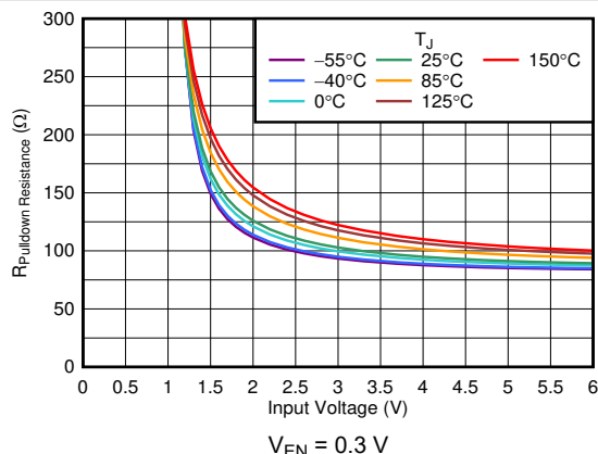
Figure 6-19. Pulldown Resistor ( R_{\text{Pulldown}} ) vs V_{\text{IN}}
