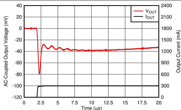
Figure 6-40. Line Transient
