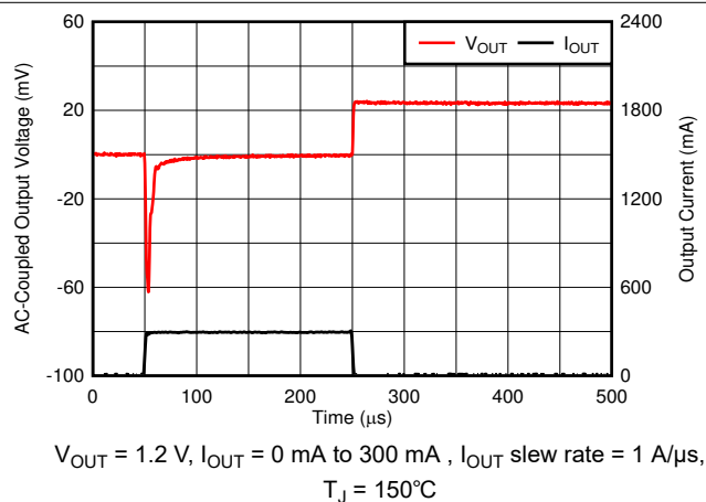
Figure 6-52. Load Transient
