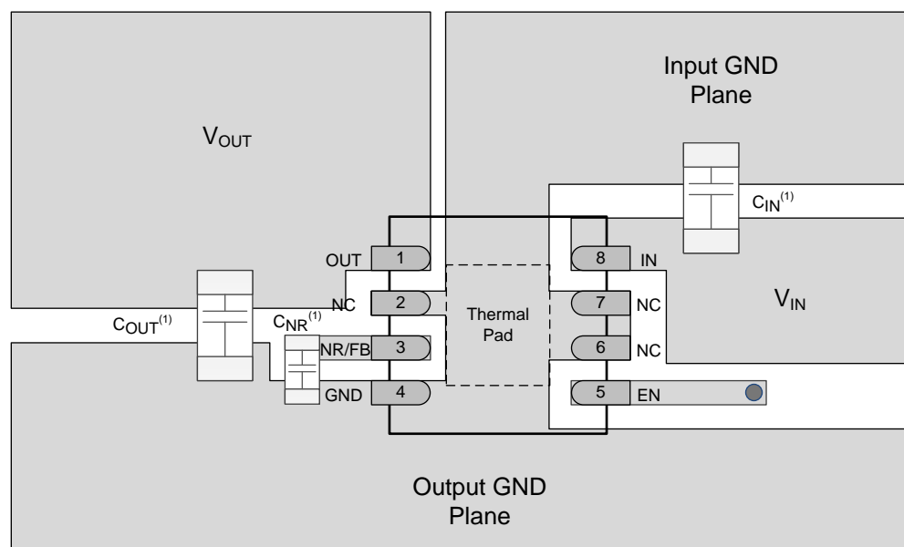
Figure 25. TPS735-Q1 Fixed Version Layout Reference Diagram
