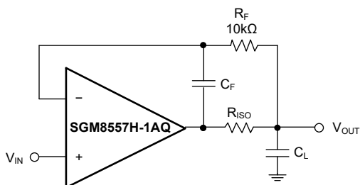
Figure 6. Circuit to Drive Capacitive Load
