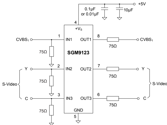
Figure 1. DC Coupling Application Schematic
