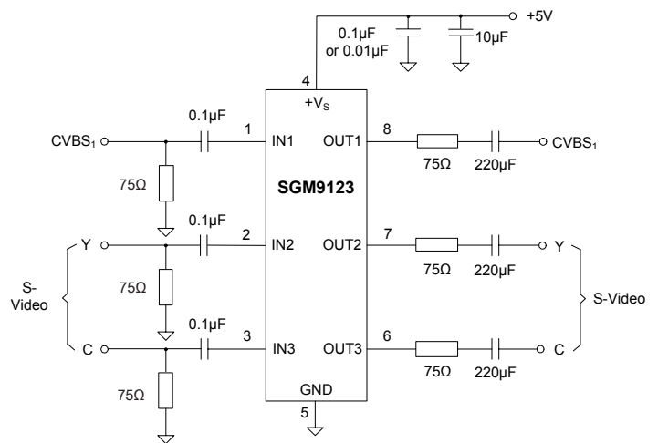
Figure 2. AC Coupling Application Schematic
