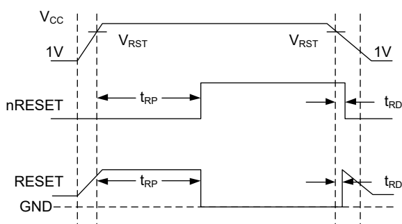
Figure 1. nRESET Timing Diagram
