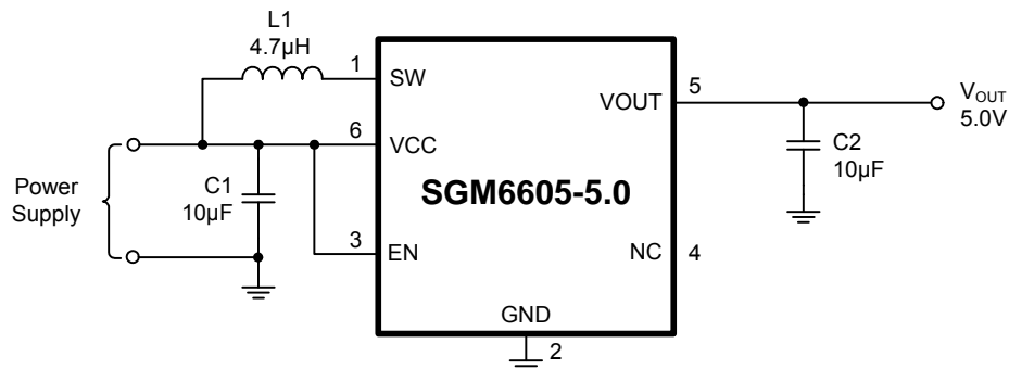
Figure 6. Basic Application Circuit for the Fixed Output Versions
