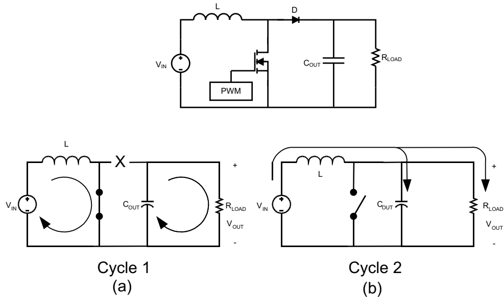
Figure 21. Simplified Boost Converter Diagram (a) First Cycle of Operation (b) Second Cycle Of Operation
