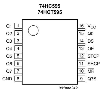
Figure 5. Pin configuration for SO16, SSOP16 and TSSOP16
