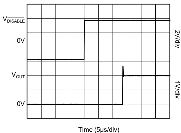
Turn-On Transient
