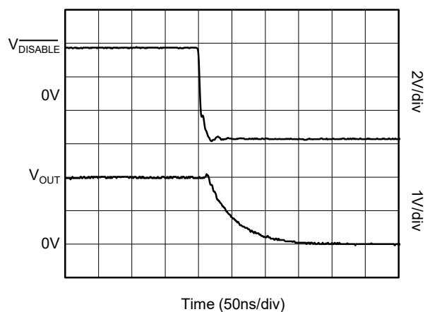
Turn-Off Transient
