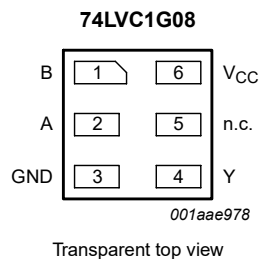
Fig. 6. Pin configuration SOT891, SOT1115 and SOT1202 (XSON6)
