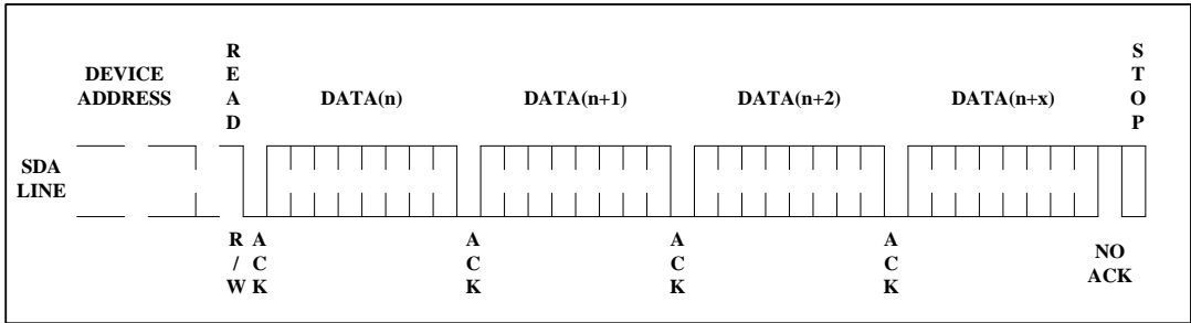
Figure 11. Sequential Read
