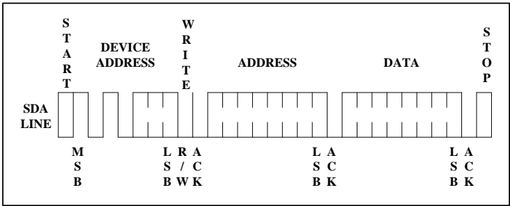
Figure 7. Byte Write
