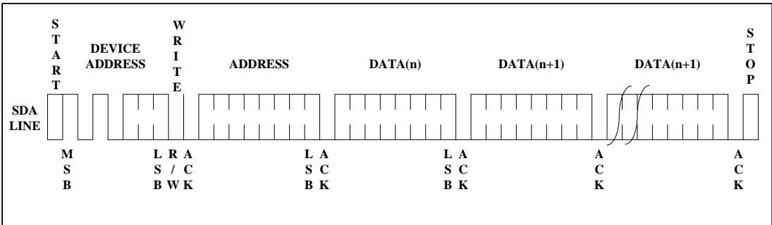
Figure 8. Page Write
