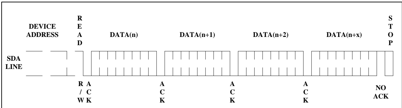
Figure 10. Sequential Read
