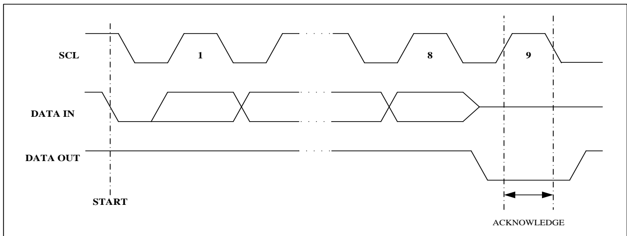
Figure 4. Output Acknowledge
