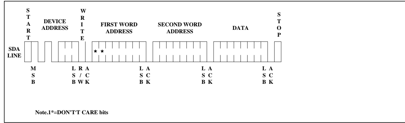
Figure 6: Page Write
