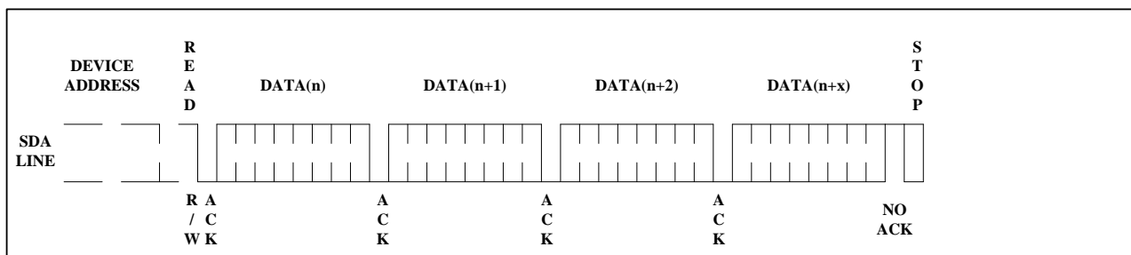
Figure 9: Sequential Read
