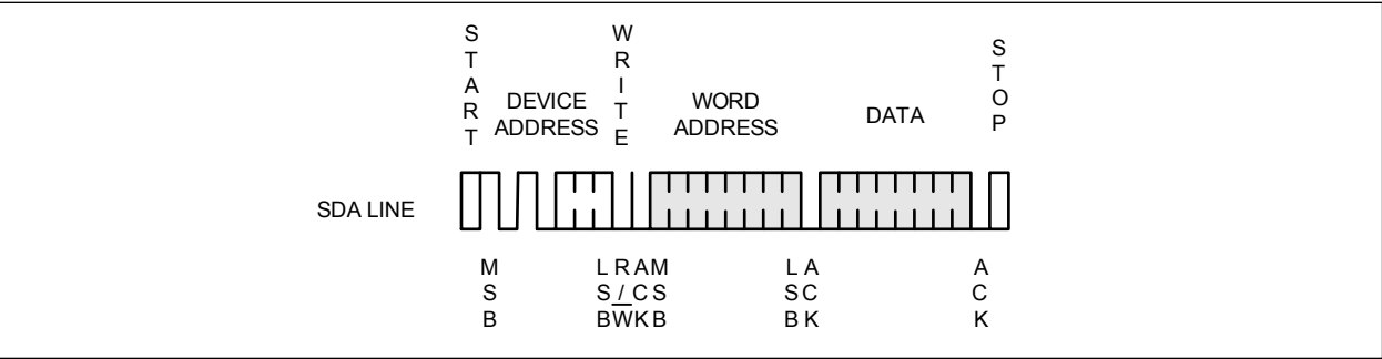
Figure 5: Byte Write
