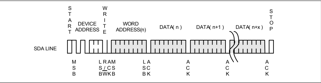
Figure 6: Page Write
