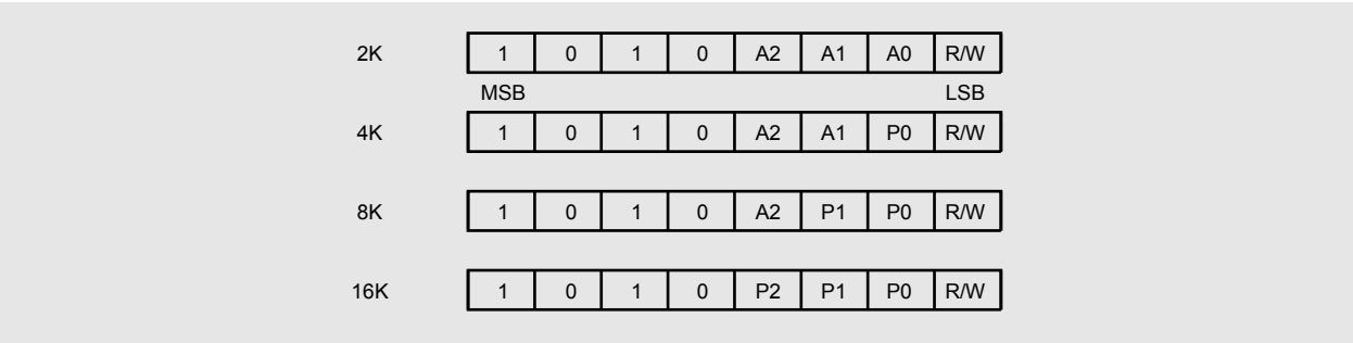
Figure 4: Device Address
