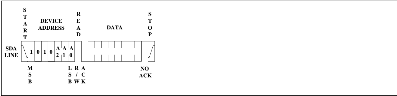
Figure 10. Random Read
