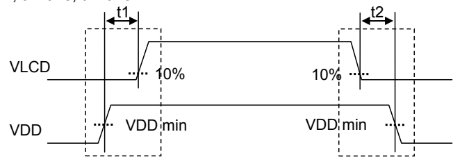
Figure 14. Power On/Off Sequence
