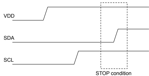
Figure 13. STOP condition
