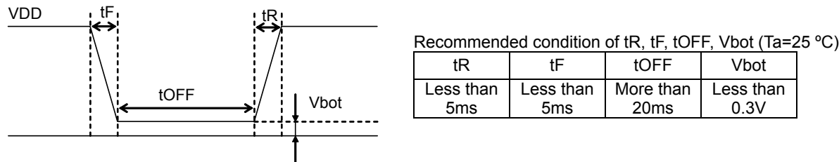
Figure 12. Power ON/OFF waveform
