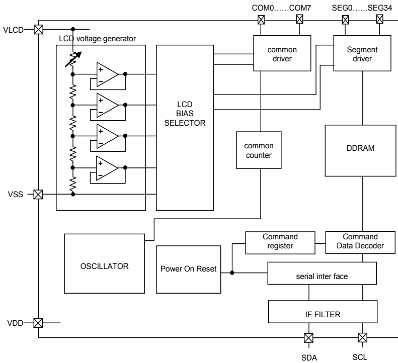
Figure 2. Block Diagram
