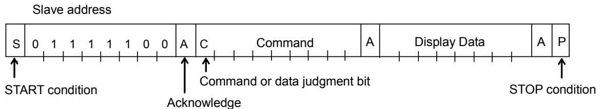
Figure 8. Interface Protocol
