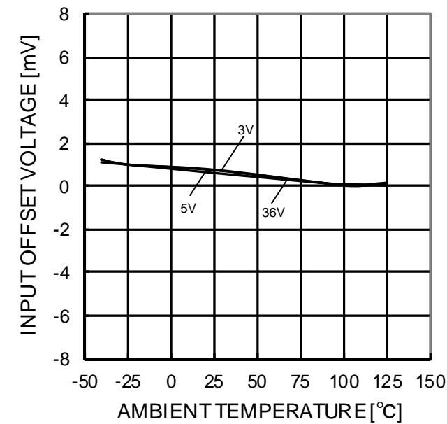
Figure 86. Input Offset Voltage - Ambient Temperature ( V_{ICM}=0V , OUT=1.4V )
