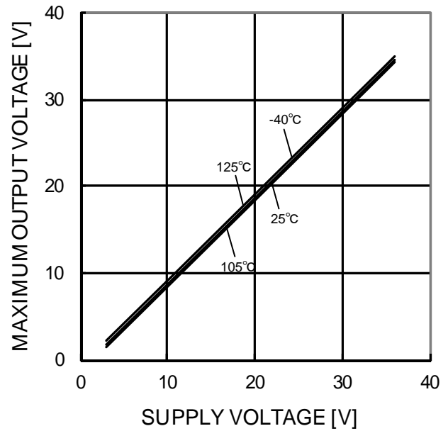
Figure 77. Maximum Output Voltage - Supply Voltage ( R_L=10k\Omega )
