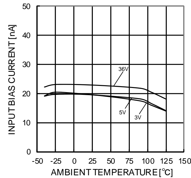
Figure 88. Input Bias Current - Ambient Temperature ( V_{ICM}=0V , OUT=1.4V )
