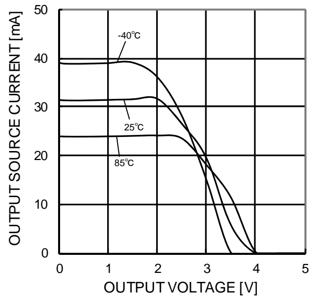
Figure 31. Output Source Current - Output Voltage (VCC=5V)
