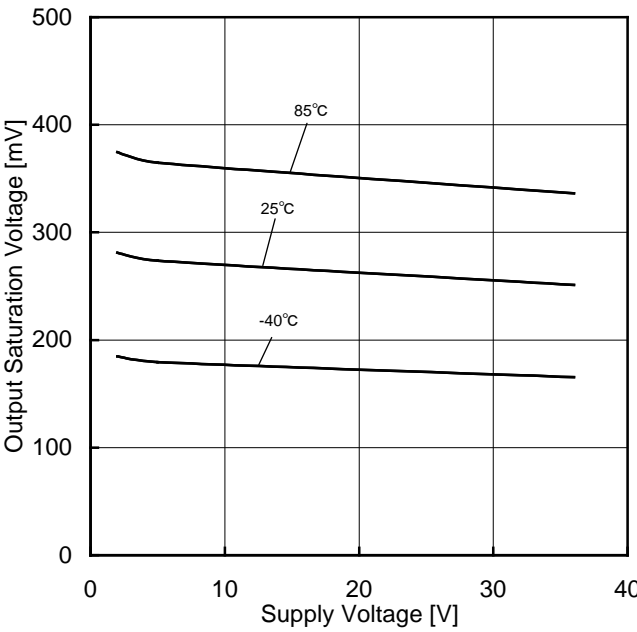
Figure 28. Output Saturation Voltage vs Supply Voltage ( I_{OL}=4mA )
