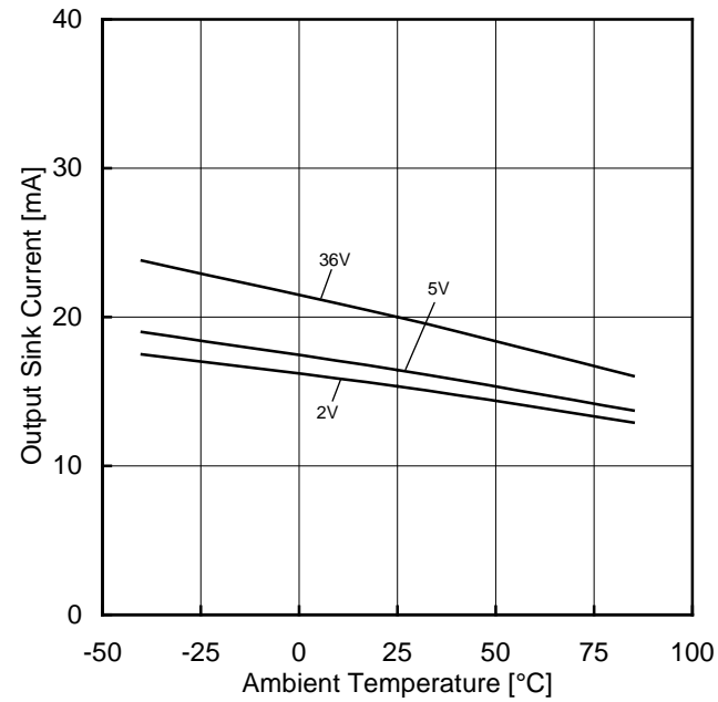
Figure 31. Output Sink Current vs Ambient Temperature ( OUT=1.5V )
