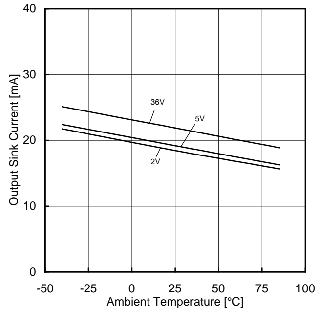
Figure 8. Output Sink Current vs Ambient Temperature ( OUT=1.5V )
