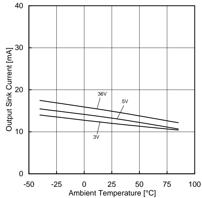
Figure 51. Output Sink Current vs Ambient Temperature (OUT=1.5V)
