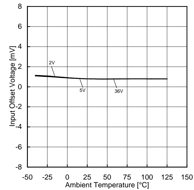
Figure 96. Input Offset Voltage vs Ambient Temperature
