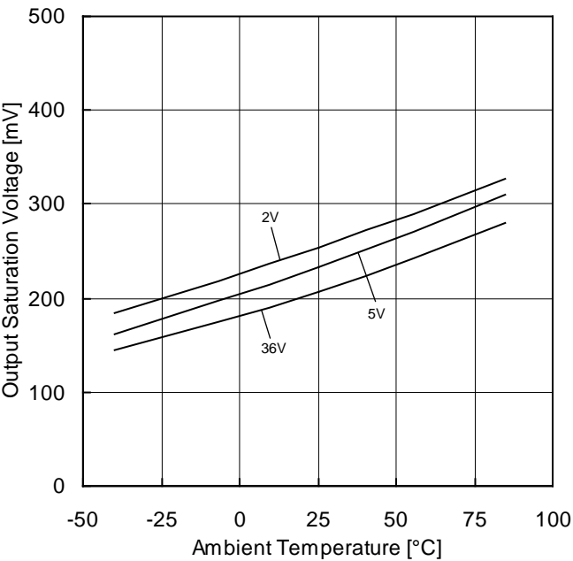
Figure 49. Output Saturation Voltage vs Ambient Temperature ( I OL =4mA)
