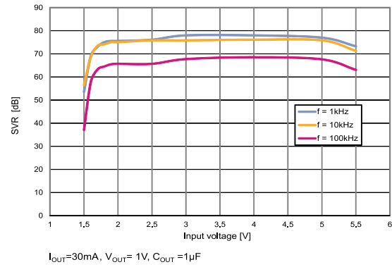
Figure 15: Supply voltage rejection vs. input voltage
