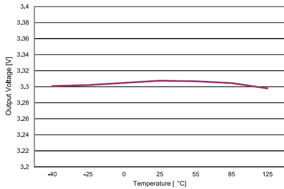
Figure 4: Output voltage vs. temperature ( I_{OUT} = 1\ mA )
