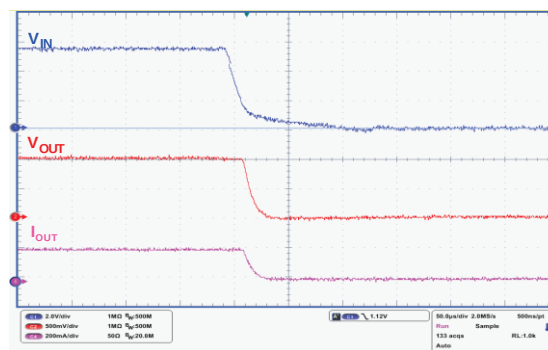
Figure 21: Turn-off time ( V_{OUT} = 1\text{ V} )
