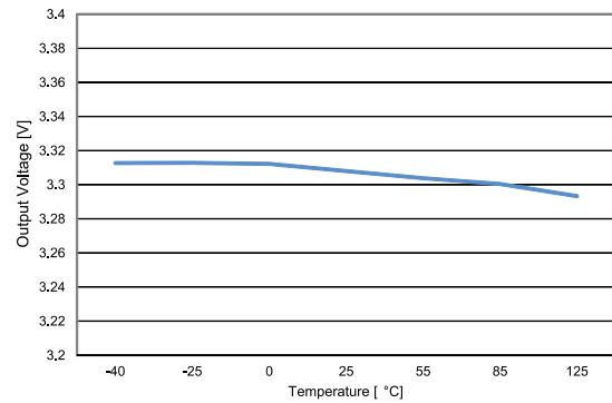
Figure 5: Output voltage vs. temperature ( I_{OUT} = 200\ mA )
