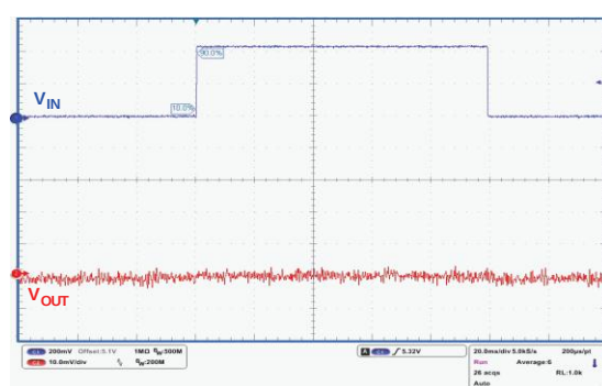
Figure 25: Line transient ( V_{OUT} = 5\text{ V} )
