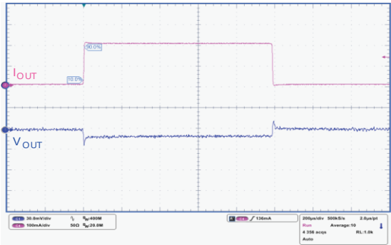
Figure 26: Load transient ( V_{OUT} = 1\text{ V} )
