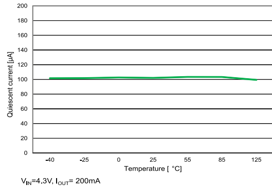
Figure 9: Quiescent current vs. temperature ( I_{OUT} = 200 \text{ mA} )
