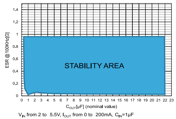
Figure 17: Stability area vs. (COUT, ESR)
