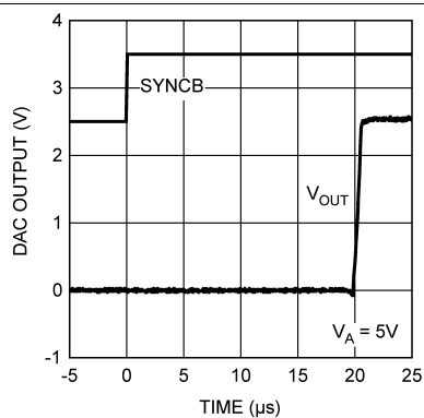
Figure 20. Settling Time
