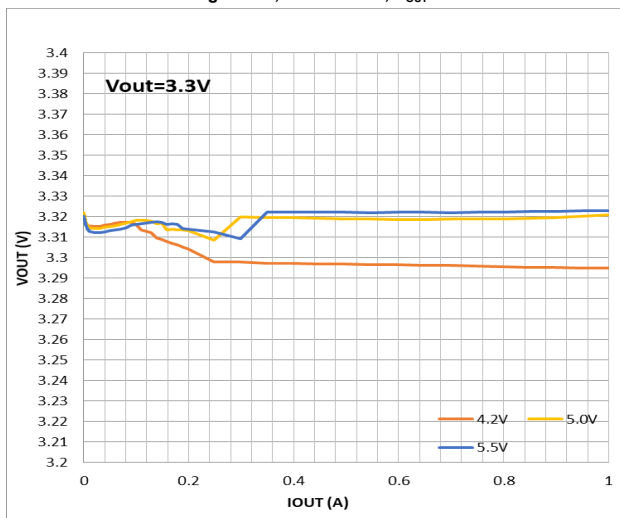
Load regulation, Mode = Low, V_{OUT} = 3.3V
