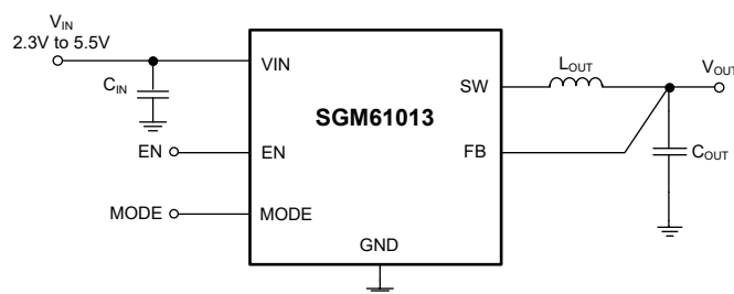
Figure 3. Application Circuit
