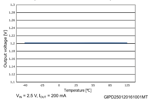
Figure 6: Output voltage vs. temperature ( V_{OUT} = V_{ADJ} , I_{OUT} = 200\ \text{mA} )
