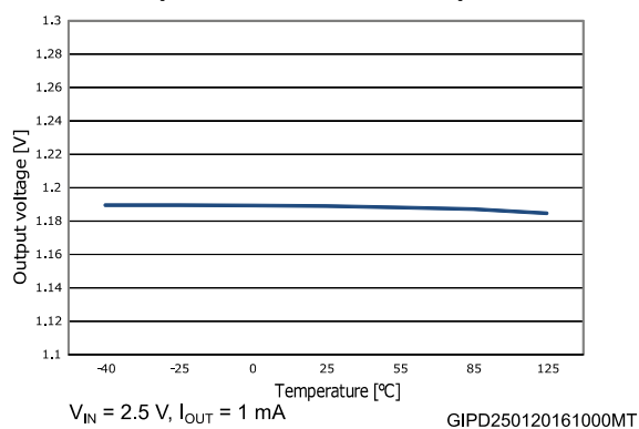
Figure 5: Output voltage vs. temperature ( V_{OUT} = V_{ADJ} , I_{OUT} = 1\ \text{mA} )
