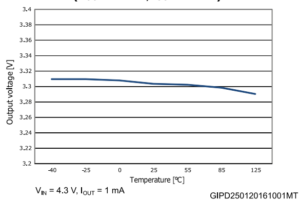
Figure 7: Output voltage vs. temperature ( V_{OUT} = 3.3\ \text{V} , I_{OUT} = 1\ \text{mA} )
