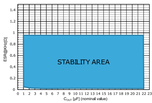
Figure 22: Stability vs. ( C_{OUT} , ESR)
