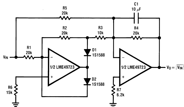
Figure 57. AC/DC Converter
