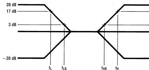
Figure 60. Tone Control
