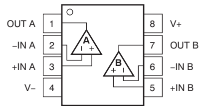
OPA2180 D, DGK Packages 8-Pin SOIC, VSSOP Top View
