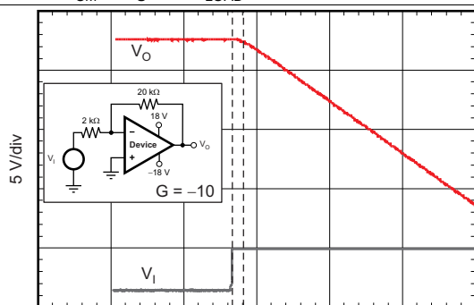
图 13. Positive Overload Recovery
