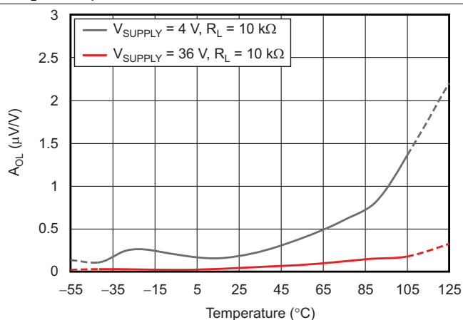
图 8. Open-Loop Gain vs Temperature
