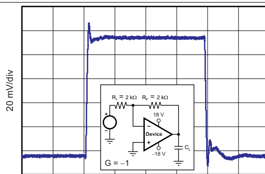
图 14. Negative Overload Recovery
