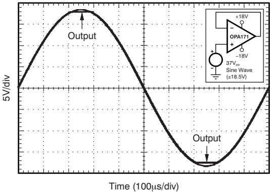
Figure 37. 无相位反转
