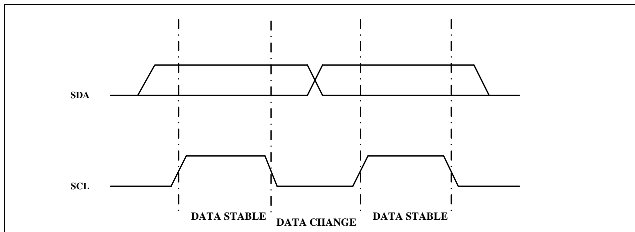
Figure 2. Data Validity
