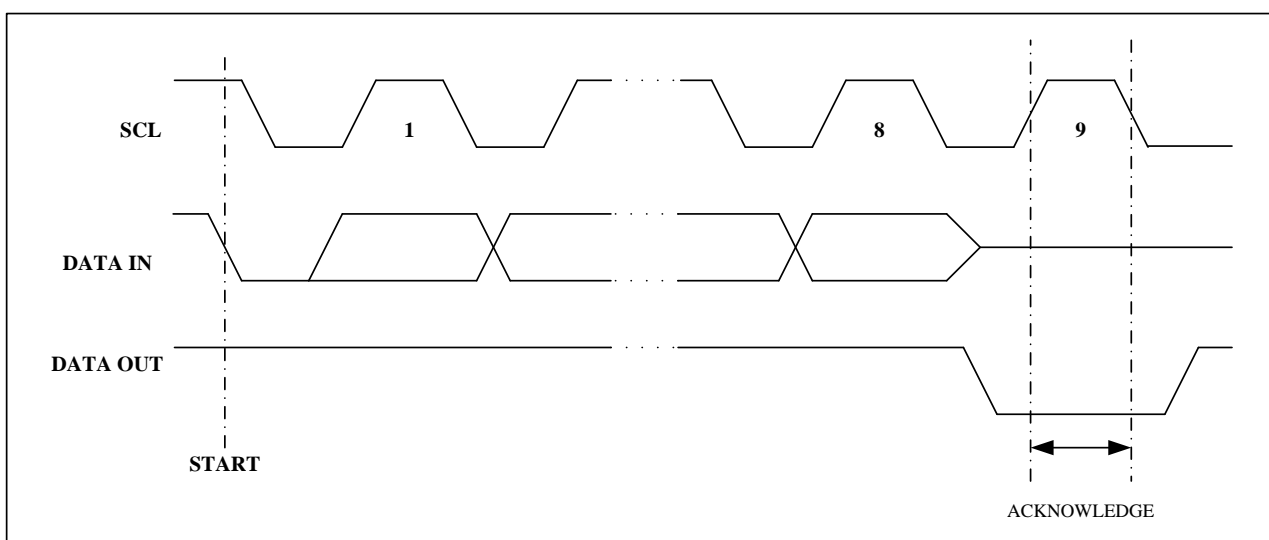
Figure 4. Output Acknowledge
