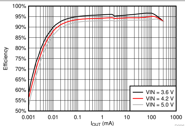
Figure 9-3. Efficiency vs Load Current, V_{OUT} = 3.3\text{ V}
