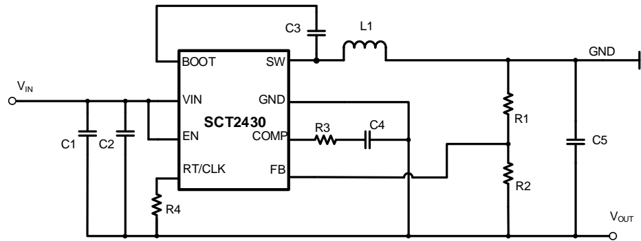
Figure 19. SCT2430 Inverting Power Supply
