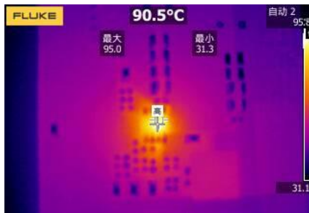
Figure 25. Thermal, 3.3Vout/3.5A
