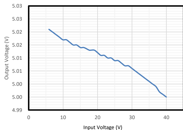
Figure 6. Line Regulation (Iout=3.5A)
