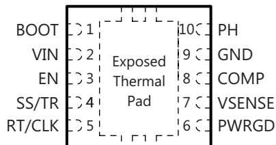
DRC Package 10-Pin VSON With Exposed Thermal Pad Top View
