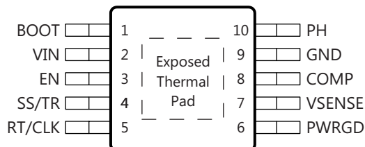
DGQ Package 10-Pin MSOP-PowerPAD Top View
