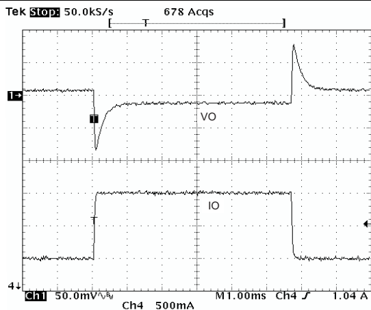
Figure 52. Load Transient
