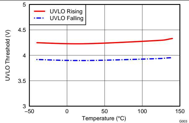
Figure 8. UVLO Threshold vs Temperature
