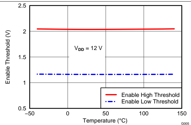
Figure 10. Enable Threshold vs Temperature
