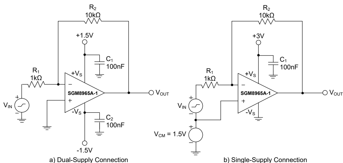
Figure 1. Basic Circuit Connections
