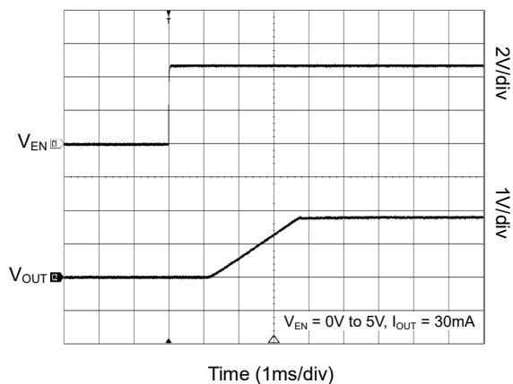
Turn-On with EN Pin
