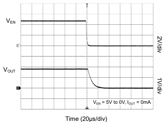
Turn-Off with EN Pin
