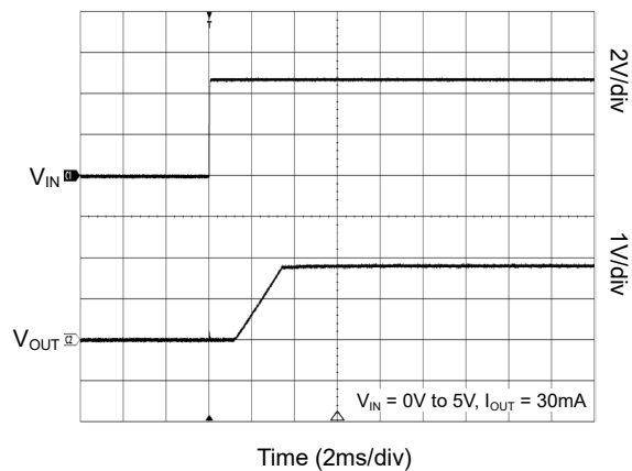
Power-Up Output Waveform
