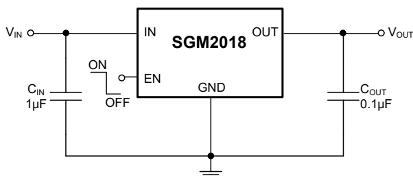
Figure 2. Application Circuit
