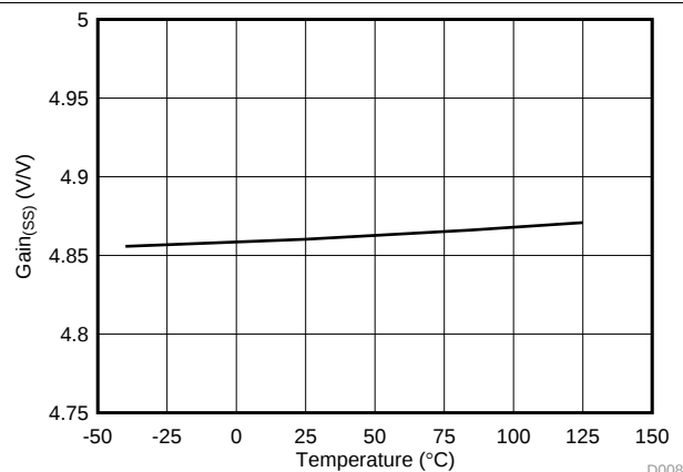
Figure 7. \text{GAIN}_{\text{(SS)}} vs Temperature
