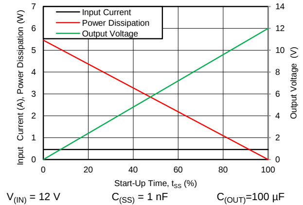
Figure 32. P_{D(INRUSH)} Due to Inrush Current
