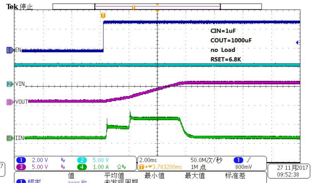
Startup from Enable ON
