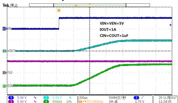
Startup from Enable ON
