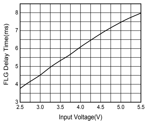
FLAG delay time vs. Input Voltage
