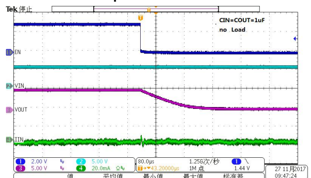
Shutdown from Enable OFF
