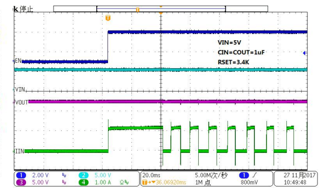
Short Circuit Response
