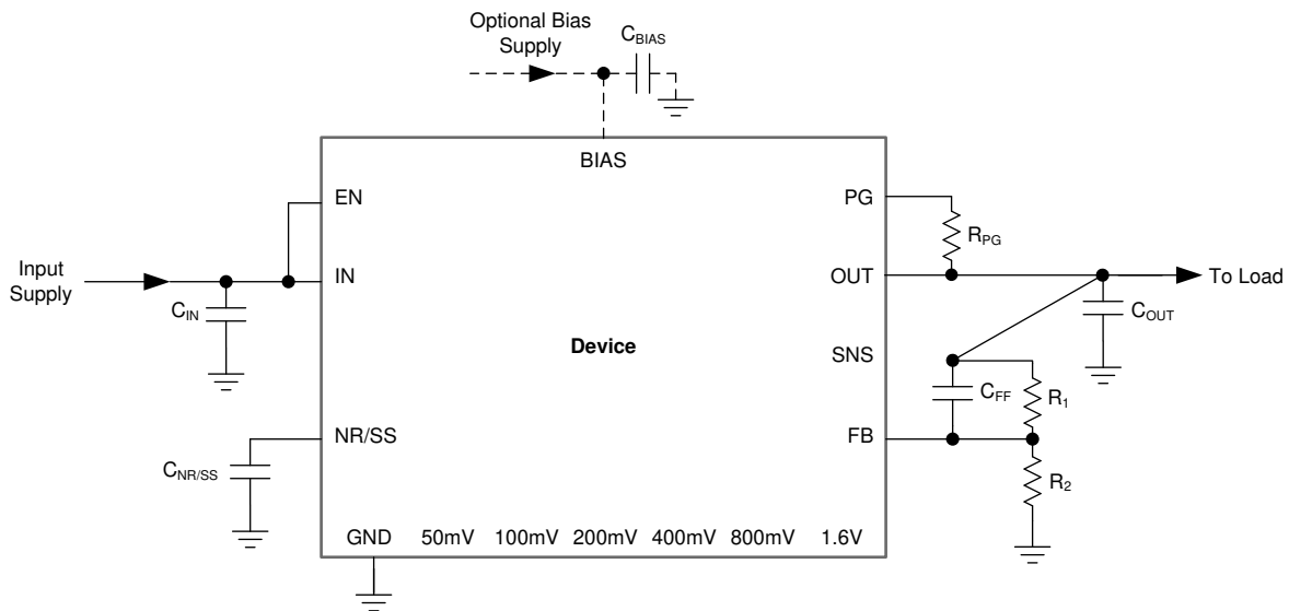
图 8-4. Adjustable Operation
