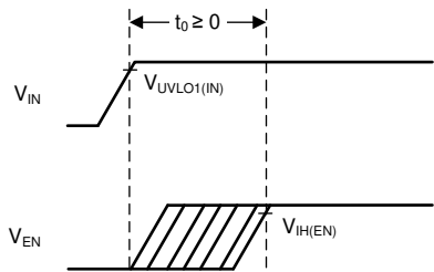
图 8-5. Sequencing Diagram
