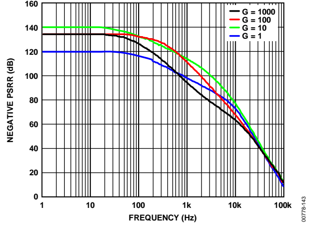
Figure 43. Negative PSRR vs. Frequency for Various Gain Settings, RM-8 and R-8 Package Options
