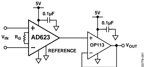
Figure 81. Output Buffering
