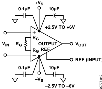
Figure 71. Dual-Supply Basic Connection
