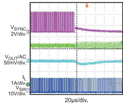
Sync Out Transient
