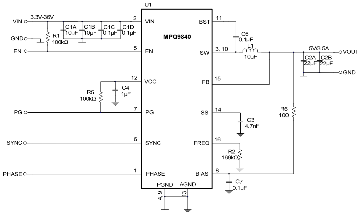
Figure 16: 5V Fixed Output, F_{sw} = 500kHz
