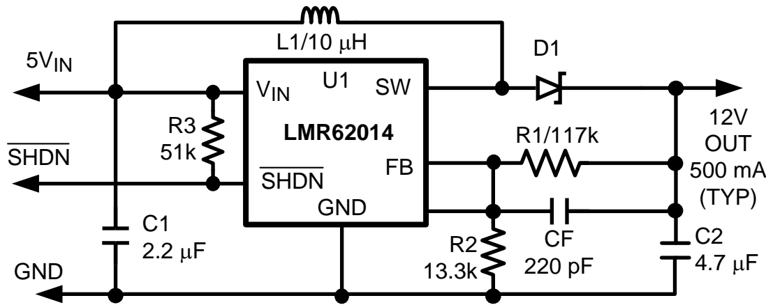
Connection Diagram
