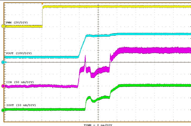
Figure 29. Start-Up with 8 Series LEDs ( D_{PWM} = 100\% )
