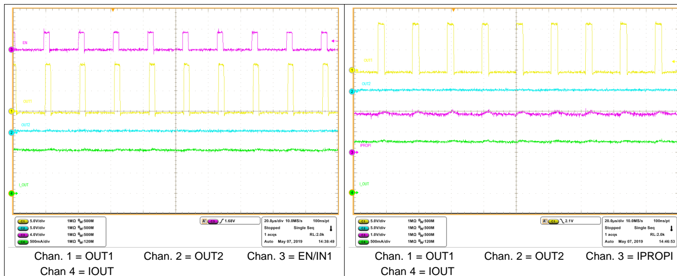
Figure 33. Driver PWM Operation (PH/EN)
