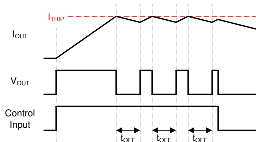
Figure 7-3. Off-Time Current-Regulation
