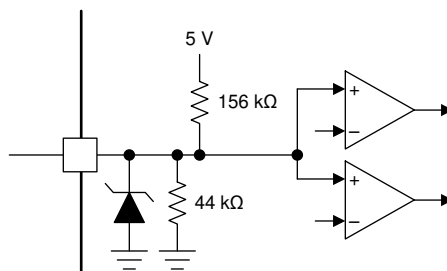
Figure 7-8. PMODE Tri-Level Input
