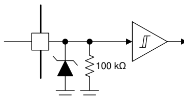
Figure 7-7. Logic-Level Input
