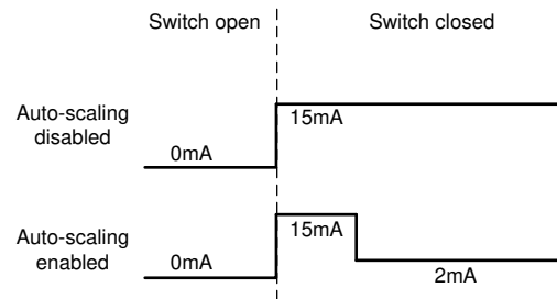
Figure 8-20. Wetting Current Auto-scaling Behavior
