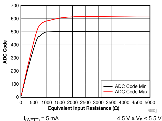
Figure 6-6. ADC Code vs. Equivalent Input Resistance
