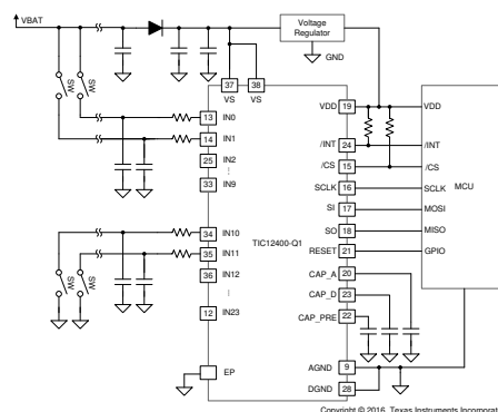
Simplified Schematic
