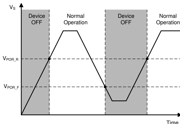
Figure 8-1. V_S is Lowered Below the POR Threshold, Then Ramped Back Up to Complete a POR Cycle
