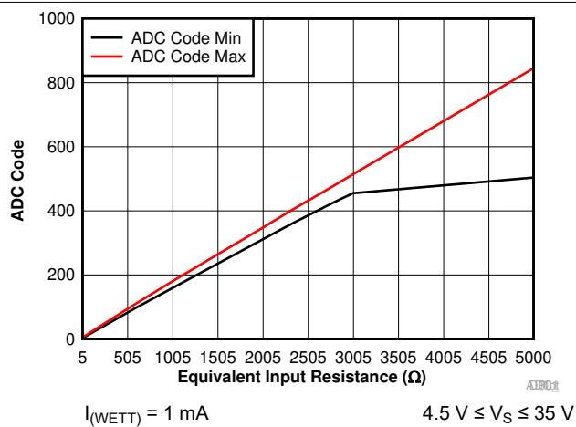
Figure 6-4. ADC Code vs. Equivalent Input Resistance
