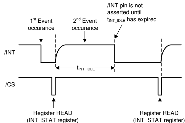
Figure 8-8. \overline{INT} Assertion Scheme With t_{INT\_IDLE}
