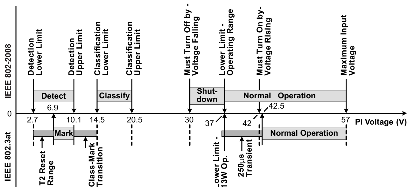
Figure 17. Threshold Voltages
