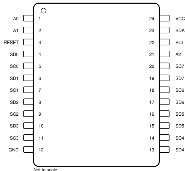
Figure 4-1. PW, DGS Package, 24-Pin TSSOP, VSSOP (Top View)
