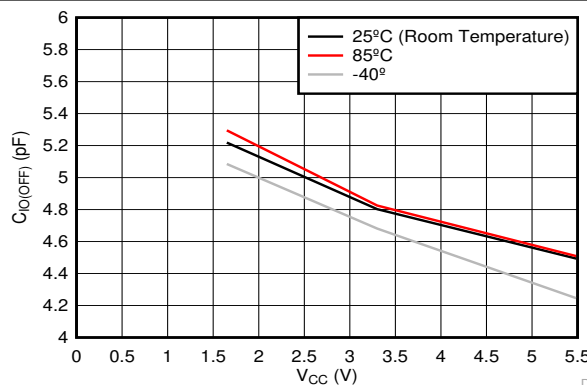
Figure 5-3. Target Channel (SCn/SDn) Capacitance ( C_{IO(OFF)} ) vs Supply Voltage ( V_{CC} ) at Four Temperature Points
