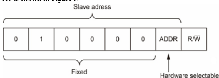
Figure 6. PI4IOE5V6416 address
