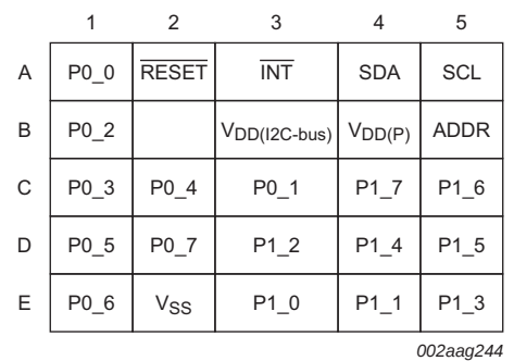
Fig 5. Ball mapping for 3 mm × 3 mm VFBGA24 (transparent top view)
