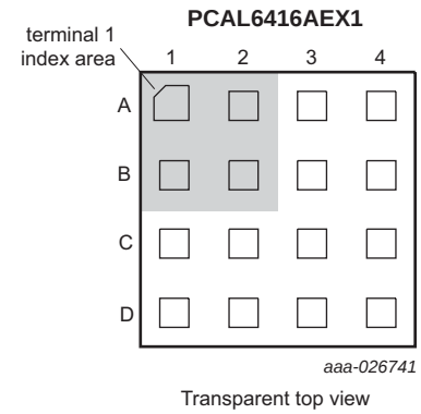
Fig 7. Pin configuration for X2QFN24 (2 mm × 2 mm); EX1 land grid array option
