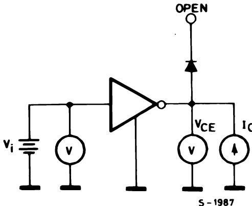
Figure 8. Input voltage
